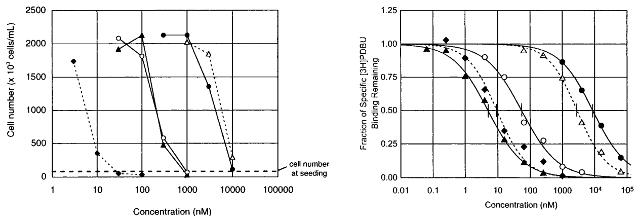
Figure 4. Biological activities of benzolactams 8 – 10 . Left: Growth inhibition of HL-60 cells. Right: Inhibition of specific [ 3 H]-PDBu binding with PKC \delta . Legend: ◆, BL-V8-310 ( 5 ); ▲, BL-8-C10 ( 8 ); ○, BL-V8-210 ( 9 ); ●, BL-V8-23TM ( 10 ); △, BL-V8 ( 4 ).
