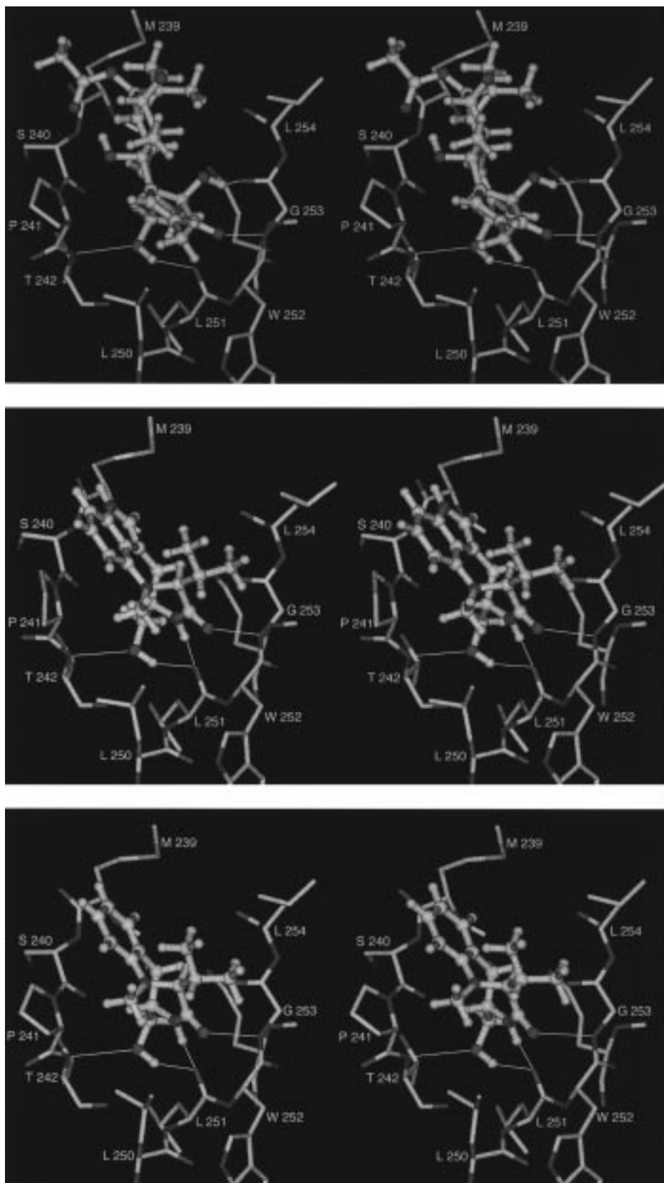
Figure 8. Stereoviews of the most stable docking models for phorbol 13-acetate (top), (-)-IL-V ( 3 ) (middle), and (-)-BL-V8 ( 4 ) (bottom). Bound ligands are shown with broad lines, and intermolecular hydrogen bonds (distances less than 3.2 Å) are shown with yellow lines.
