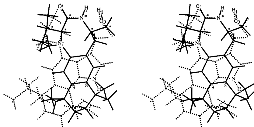
Figure 6. Molecular superposition of teleocidin B-4 ( 1 ) (dotted line) and (-)-BL-V8-23TM ( 10 ) (solid line). The two molecules were superposed on the basis of root-mean-square fit of the pairs of atoms marked with asterisks.
