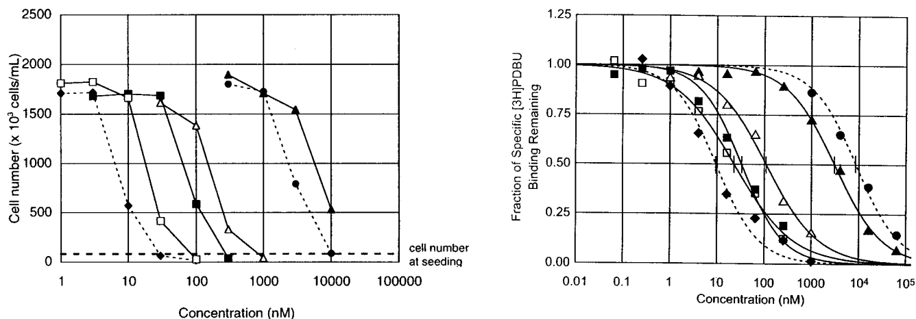
Figure 7. Biological activities of hydrophobically modified benzolactams 35–38 . Left: Growth inhibition of HL-60 cells. Right: Inhibition of specific [ 3 H]PDBu binding with PKC \delta . Legend: \blacklozenge , BL-V8-310 ( 5 ); \triangle , BL-V8-DM1 ( 35 ); \blacktriangle , BL-V8-DM3 ( 36 ); \blacksquare , BL-V8-SP1 ( 37 ); \square , BL-V8-SP3 ( 38 ); \bullet , BL-V8-23TM ( 10 ).
